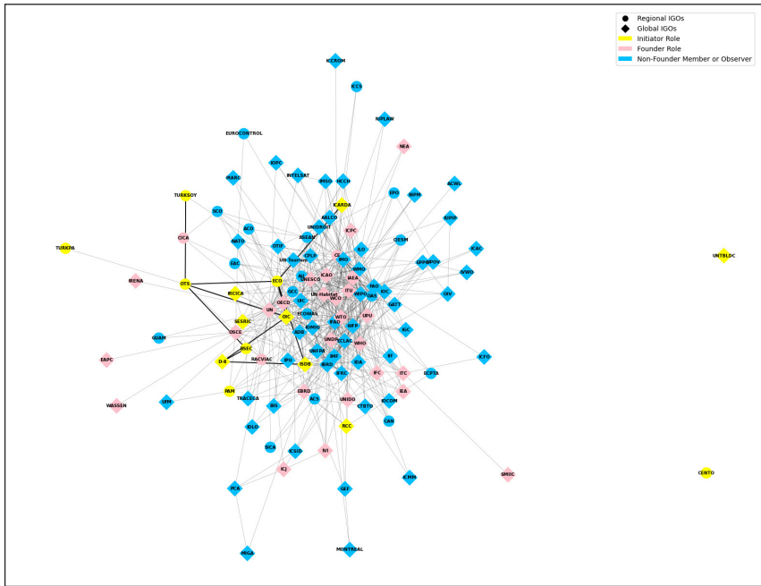
Figure 4. A network graph of bilateral legal relations between IGOs with the membership of Türkiye (Source: Union of International Associations (UIA), Graph is the authors' own production).
